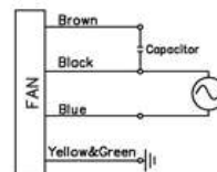
Wiring Diagram
