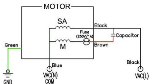
ACF19070-HL Wiring Diagram
