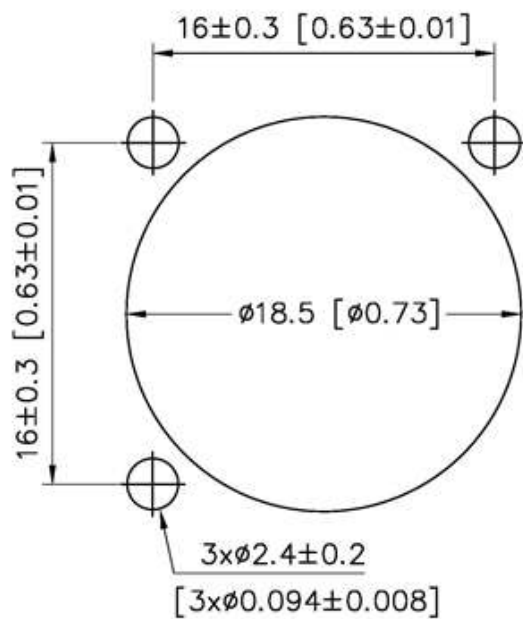
Mounting Panel Cutout Outlet Side & Inlet Side
