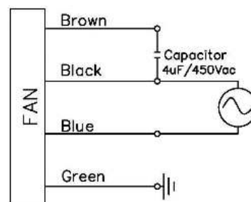
Wire Diagram
